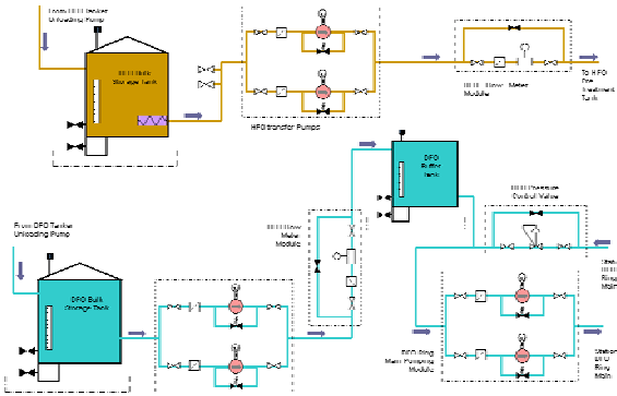
Typical Station Bulk Fuel Storage System
