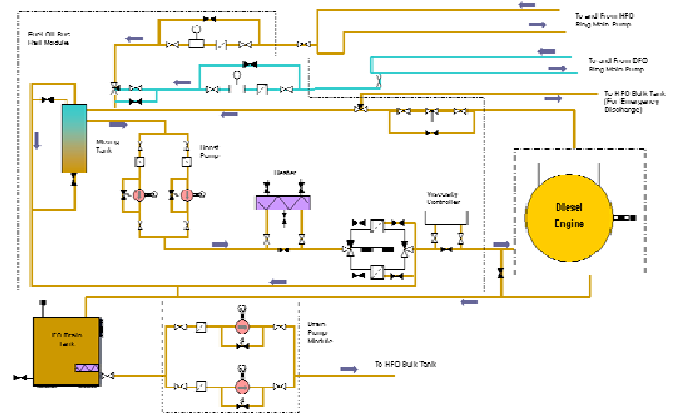
Typical Engine Fuel Oil System
